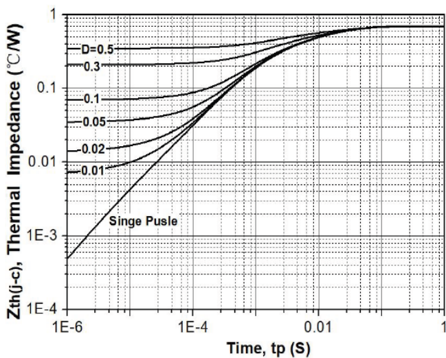
Figure 19. Transient thermal impedance (junction - case)
