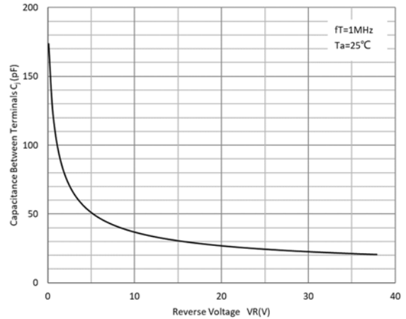
Fig 2: Capacitance Capability
